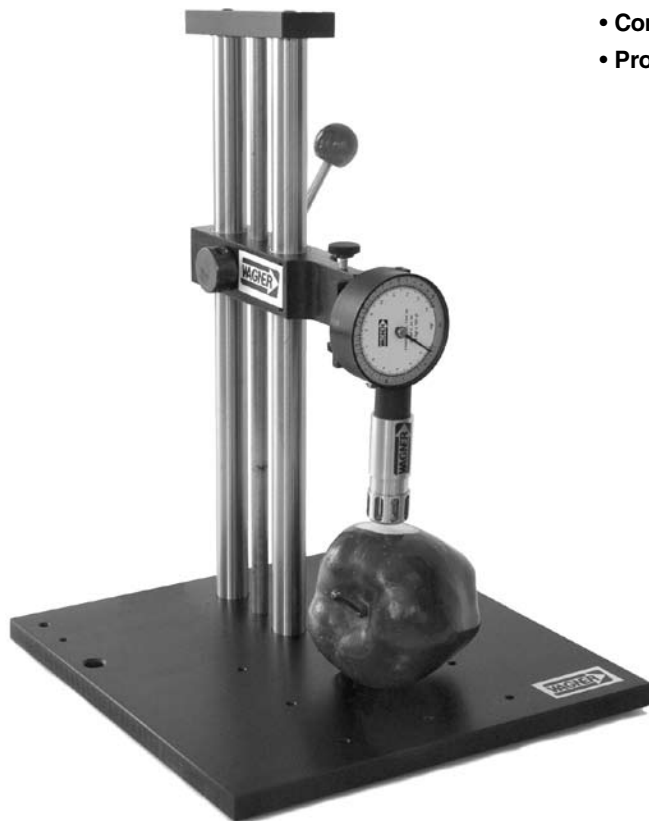
FTX Extra Mounted on FTK 100 Test Stand
